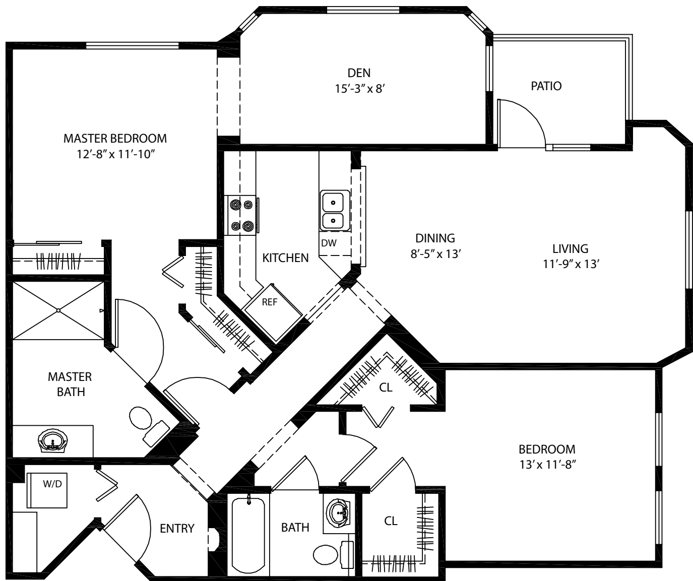
2 Bedroom/Den/2 Bath 1,200 Sq.Ft Patio: 52 Sq.Ft
